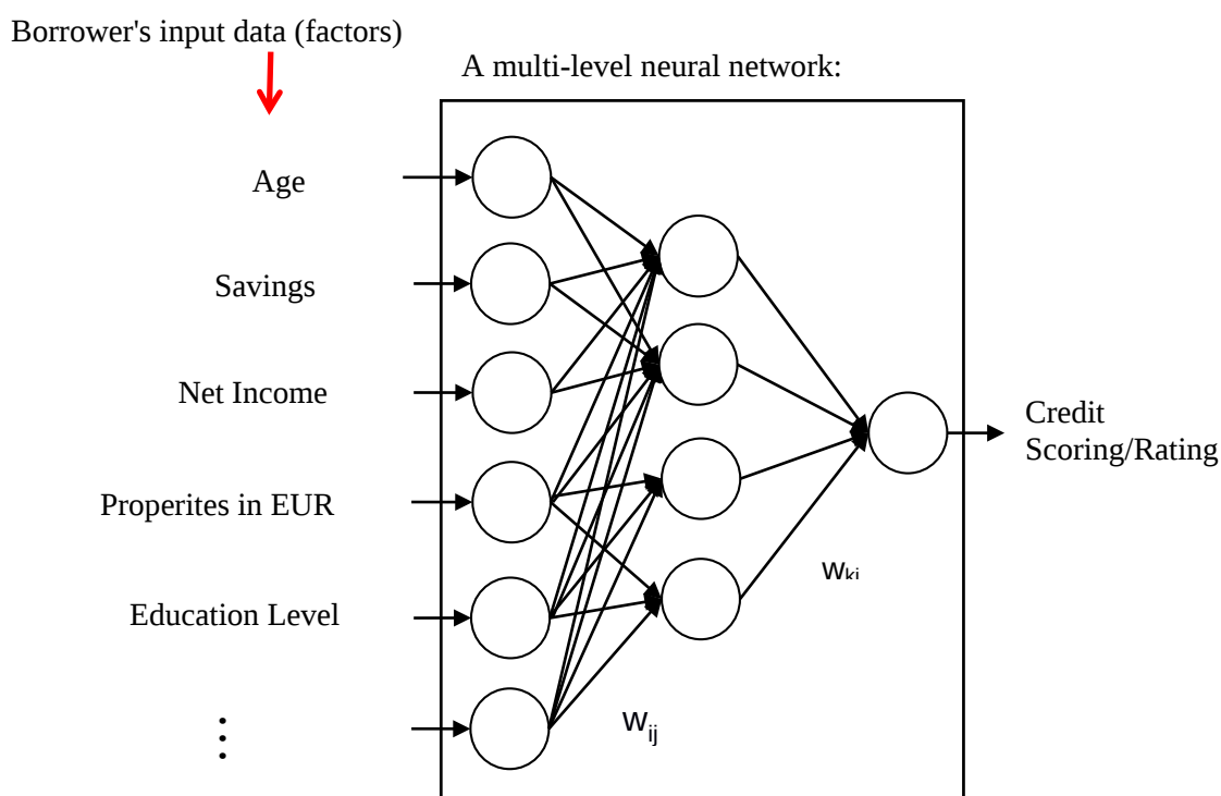
Fig. 1. Structure of a neural network
