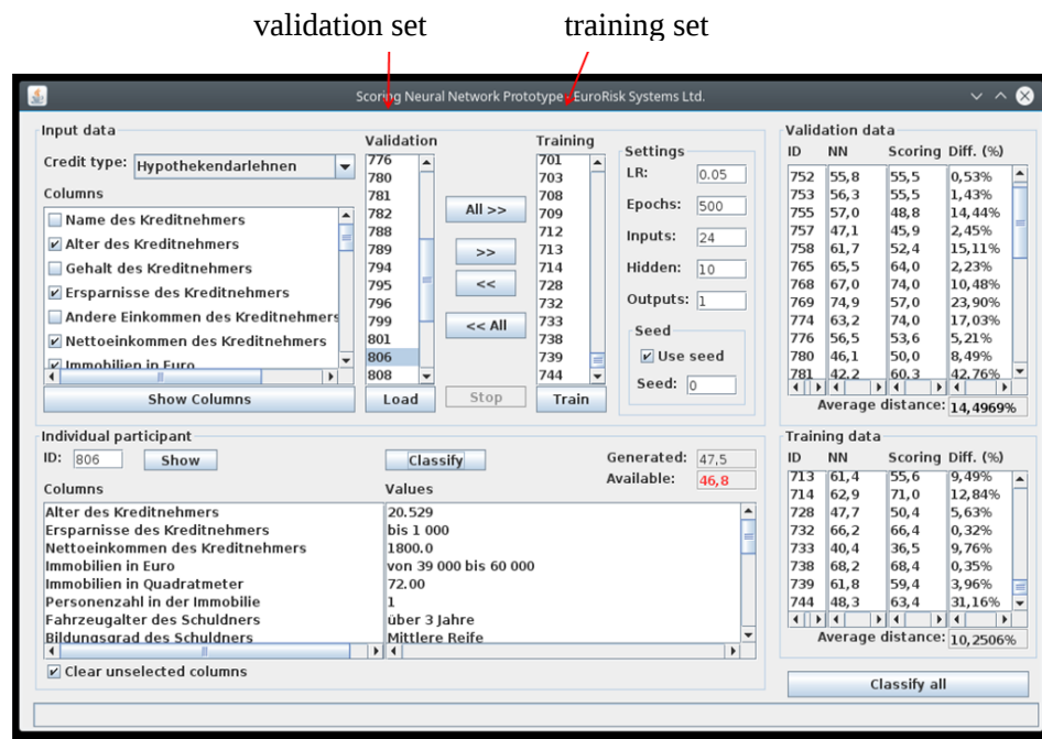
Fig. 5. Prototype of the neural network: training and scoring of new mortgage loans
