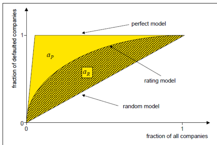
Fig. 8. CAP (Cumulative Accuracy Profile)
