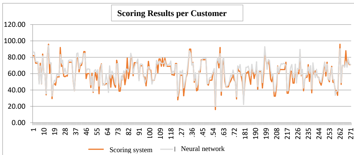
Fig. 6. Scoring system versus neural network
