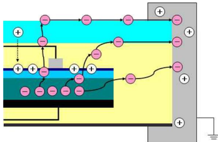
Fig. 4. Schematic indication of the charge flow leading to the PID process
