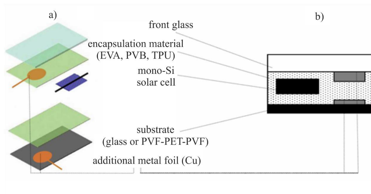
Fig. 5. Configuration of the tested photovoltaic samples
