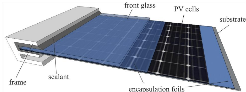
Fig. 2. Structure of a thin-film photovoltaic module
