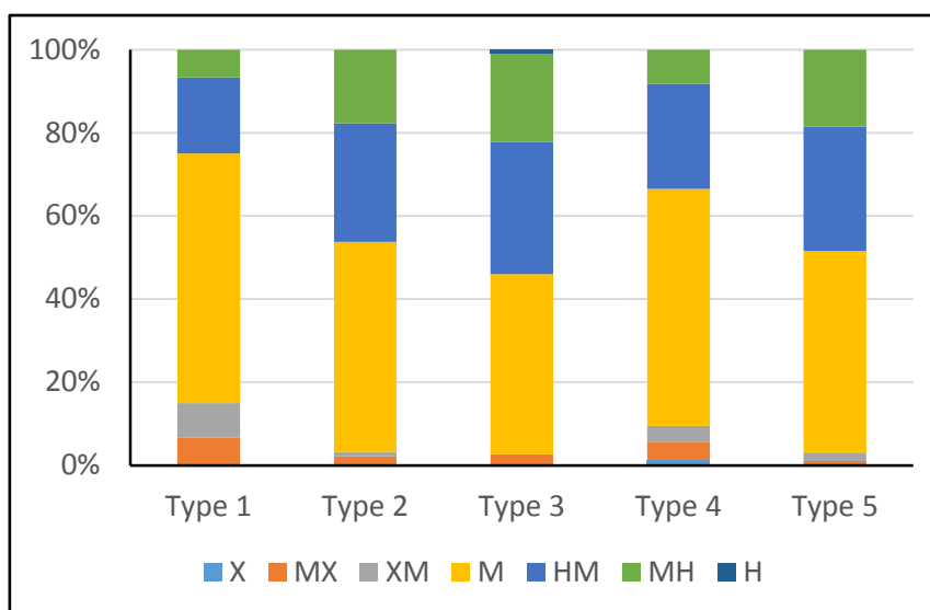
Fig. 3. The spectra of ecological (humidification) groups of species of forest types.
